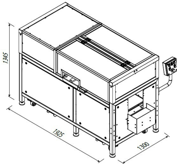
Box feeding through the top
